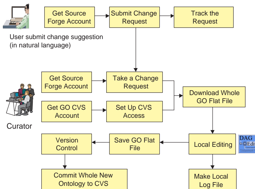
Figure 7.3 Collaborative Ontology Building with CVS: Gene Ontology
