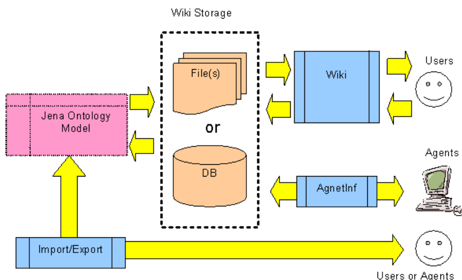
Figure 7.6 The Architecture of WikiOnt
