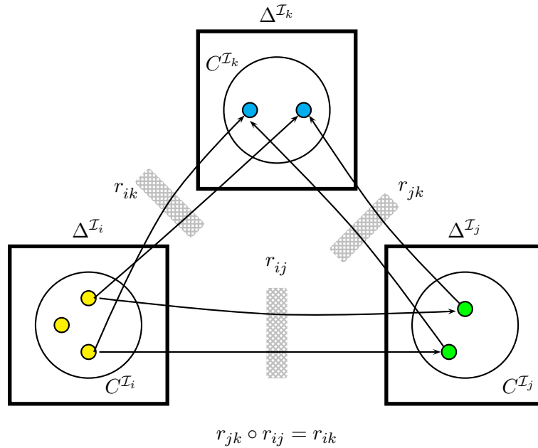
Figure 4.2 Compositionally Consistent Domain Relation
