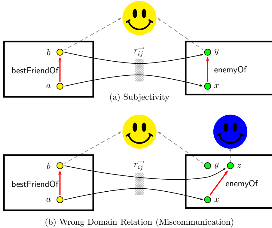
Figure 3.11 Two Types of Inconsistencies between Agents
