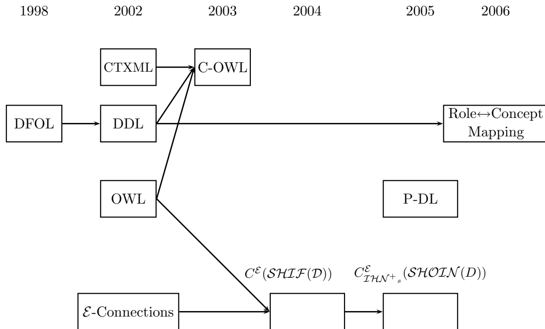
Figure 4.4 Evolution of Modular Ontology Languages
