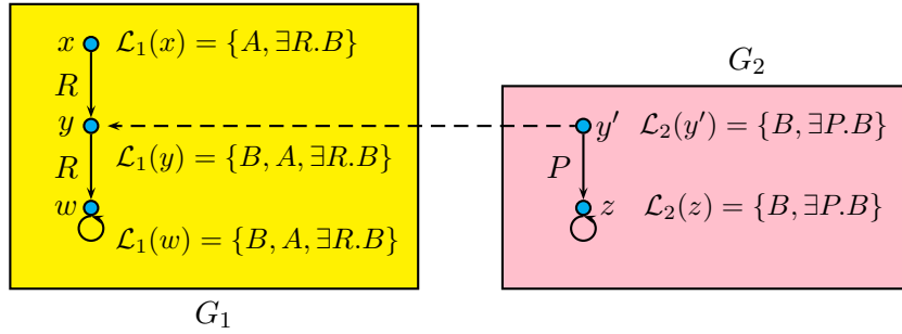
Figure 5.2 Subset Blocking Example in \mathcal{ALCP}_C^-
